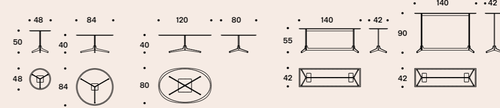
Top tondi / Round top
