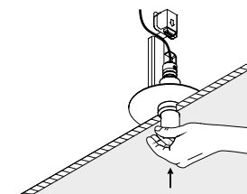
PLASTERBOARD FLANGE IP65
